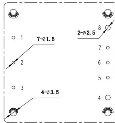
Recommended PCB Slot size
