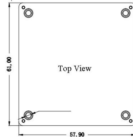
Standard 61*57.9*12.7mm
