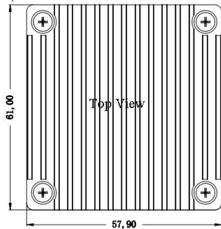
Standard+Heatsink 61*57.9*27.7mm
